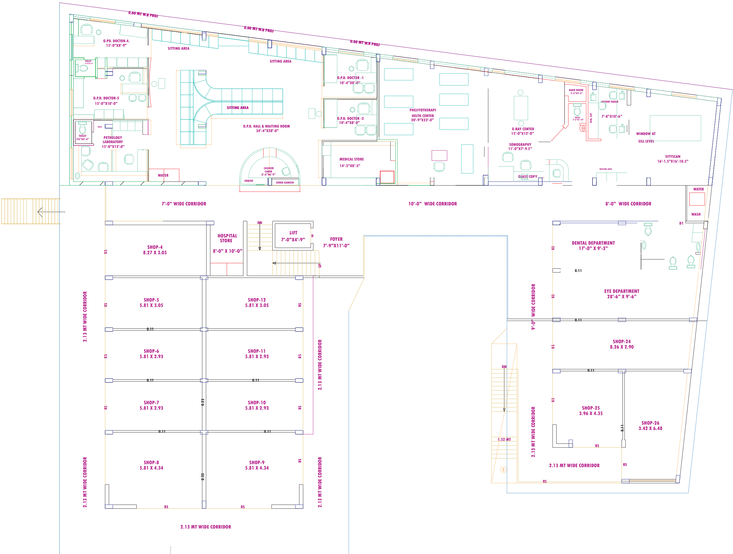
UFIRST FLOOR PLAN.(PROP. HOSPITAL)
